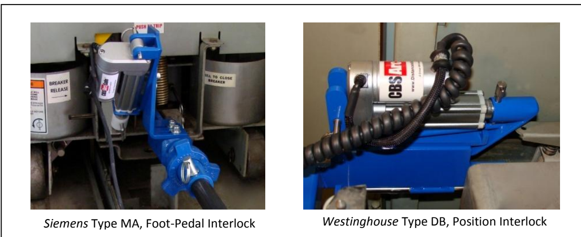
Figure 1.5 – Interlock Actuators and Tooling
